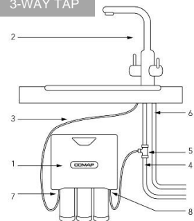
3-WAY TAP
